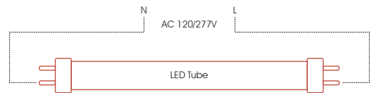
Type B-Double Ended Input
